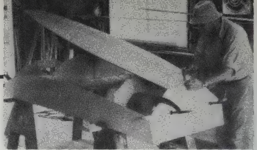
Tacking on the bottom panel. The stern transom is stiffened temporarily with a batten, and an oar holds up the forward end of the bottom panel while the after end is tacked.
